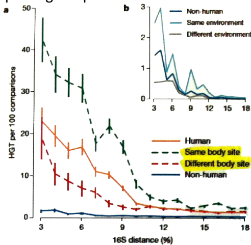
Figure 1 | Recent HGT is enriched in the human microbiome across all phylogenetic distances. HGT frequency is plotted as a function of the phylogenetic divergence between species for human-associated bacteria (a) and non-human-associated bacteria (b). We define species as clusters of genomes separated by less than 2% 16S rRNA divergence. HGT frequency is calculated in bins of 1% 16S rRNA divergence. Error bars indicate s.d. (see Supplementary Methods), with sample sizes described in Supplementary Table 8. These trends are also observed after controlling for the potential effects of sequencing centre contamination (Supplementary Fig. 4) and cosmopolitan strains (Supplementary Fig. 6).
